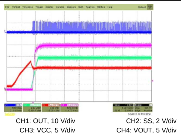
Figure 21. 230-V Start-Up, 0.1-A Load
